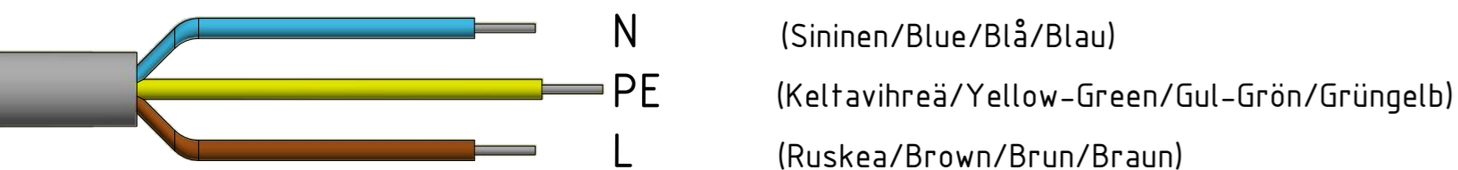
D ( 1 : 1 ) (3x1,5mm 2 )
