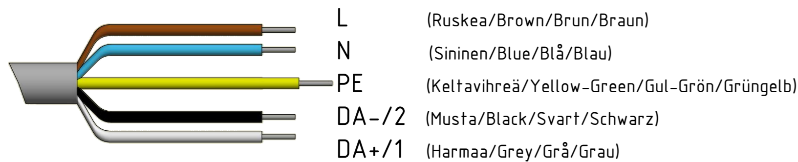
D ( 1 : 1 ) (5x1,5mm 2 )
