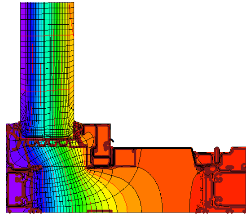
Isothermal
