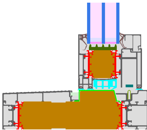
Calculation model
