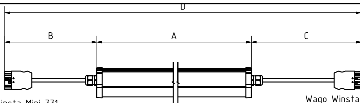
Wago Winsta Mini 771 MALE connector (5x2,5mm 2 )
