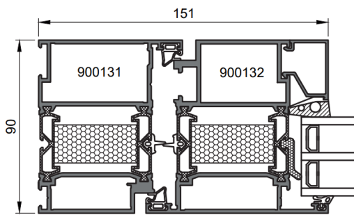
Pic 1. Old LK90H cross section
