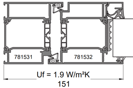
Pic. 4. LK78Xe (Same than LK78X, but without PUR and QLon -insulation)
