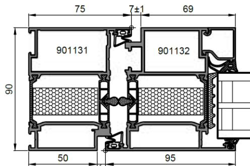
Pic 2. New LK90X cross section
