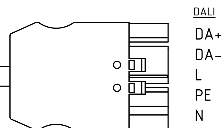
WAGO Winsta Midi 771 MALE connector (5x2,5mm 2 )
