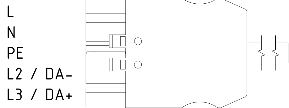
Wago Winsta Mini 771 MALE connector (5x2,5mm 2 )
