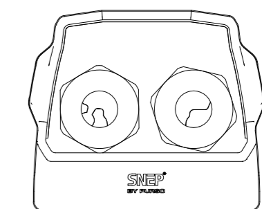
=C25 =C25DA max 5x2,5m2 Ø 8-17 mm
