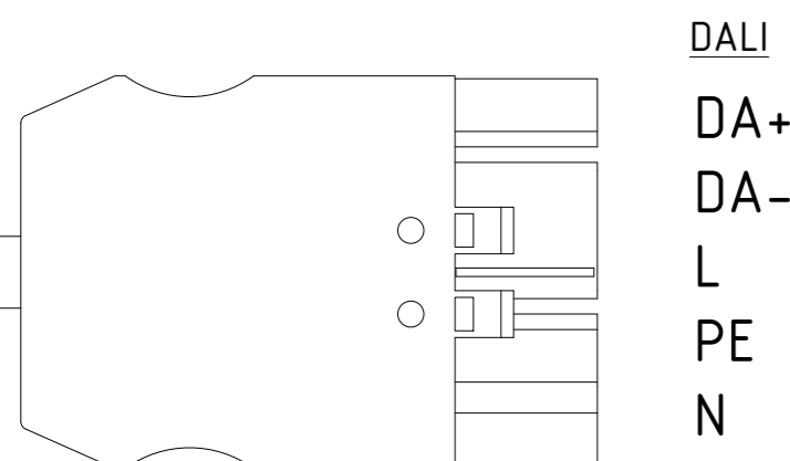
WAGO Winsta Midi 771 MALE connector (5x2,5mm 2 )
